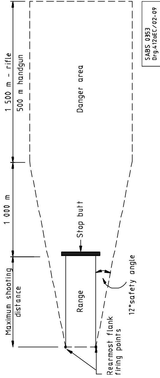
Figure 1 – Outdoor danger area range (danger area template)
